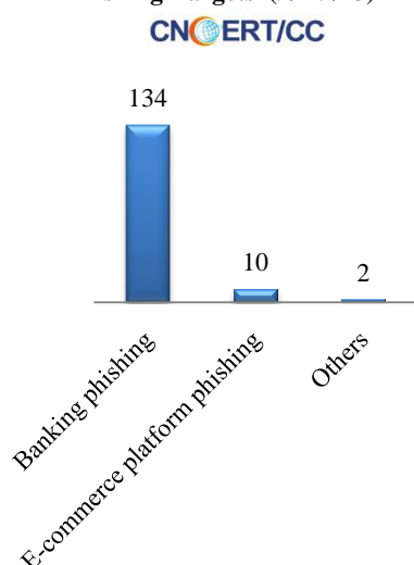
Phishing Incidents Handled by CNCERT Based on Industries of the Phishing Targets (9/7-9/13)
